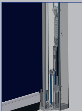
Weight compensation and permanent curtain tension
