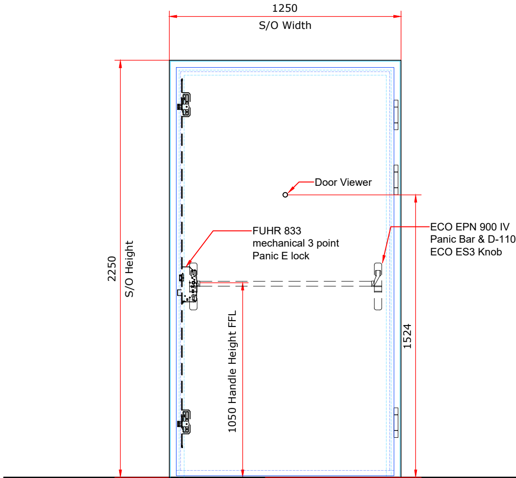
Elevation From Hinge Side
