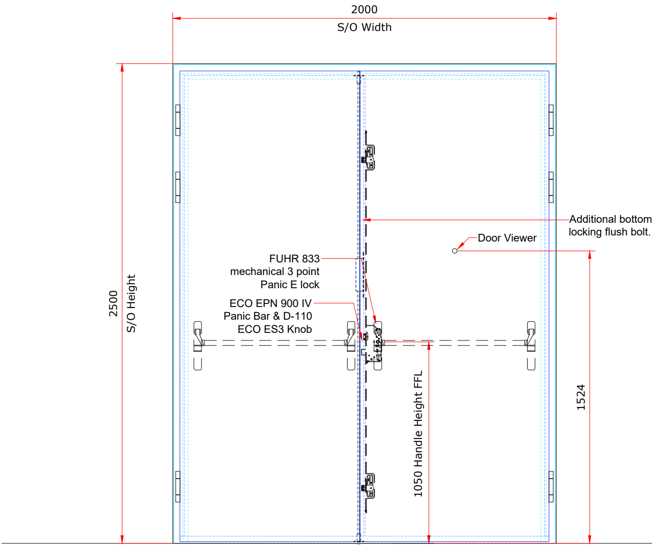
Elevation From Hinge Side
