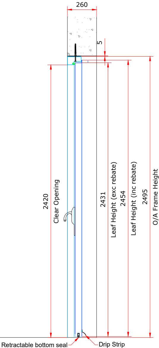
Section View
