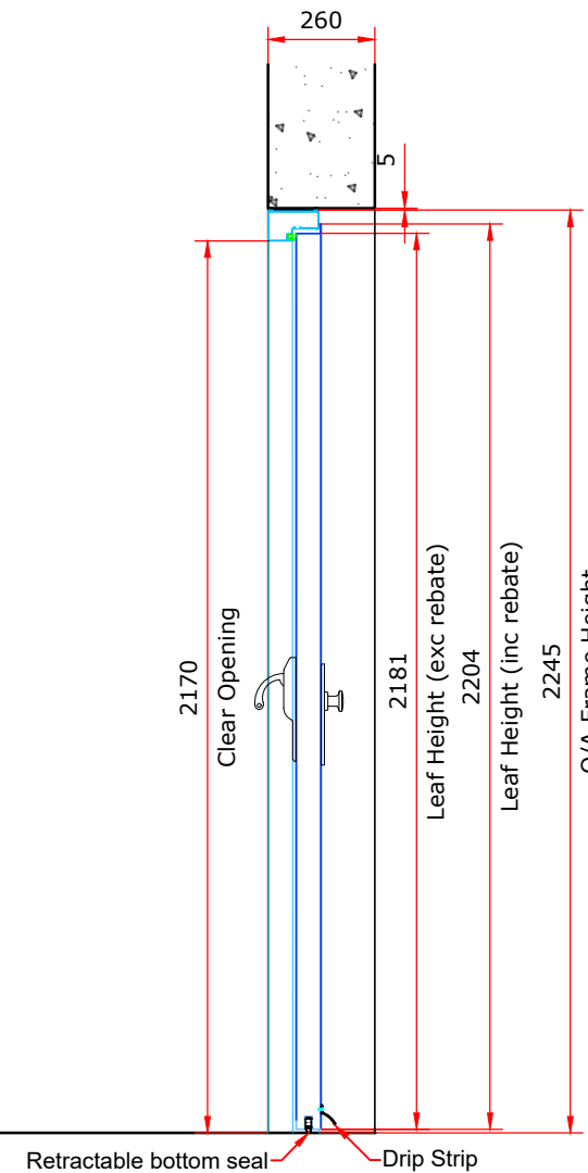
Section View
