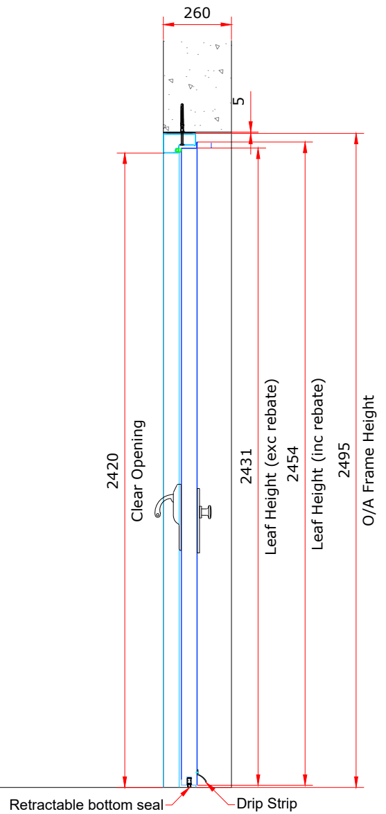
Section View
