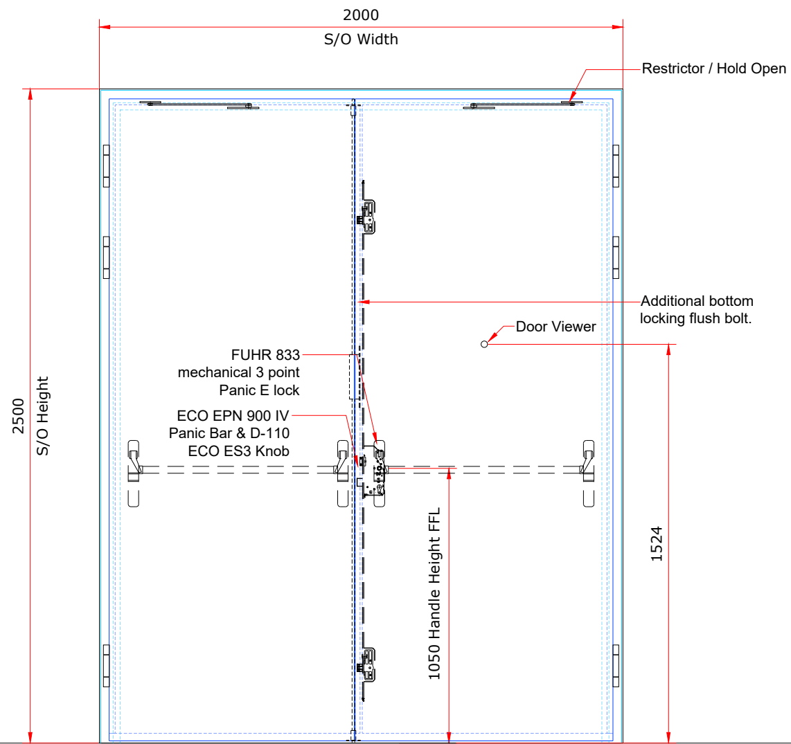
Elevation From Hinge Side
